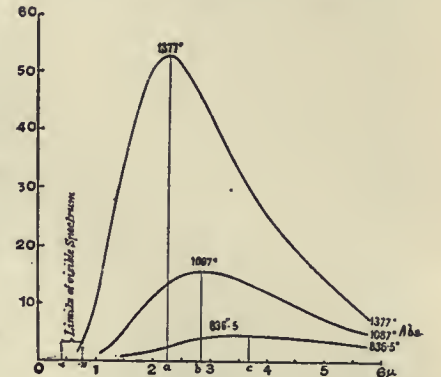
FIG. 7.—Distribution of energy in the spectrum of a black body.
